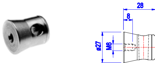
6011-002-002 ( 601116 ) MALE HALF CONNECTION
