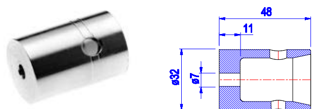
6011-001-002 ( 601118A ) FEMALE CONNECTION Ø7 L=48
