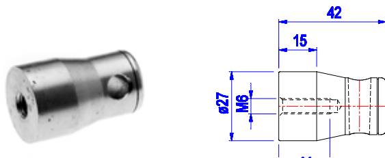
6011-002-004 ( 601119 ) MALE HALF CONNECTION M6 +15MM
