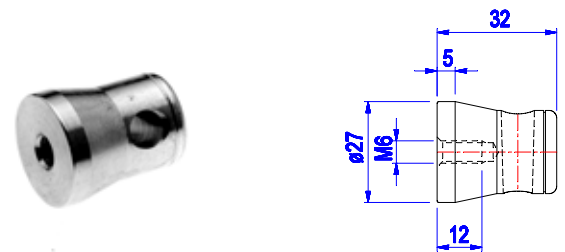
6011-002-003 ( 601117 ) MALE HALF CONNECTION M6 +5MM
