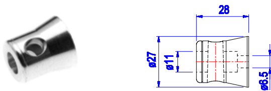
6011-002-005 ( 601122 ) MALE HALF CONNECTION Ø6,5
