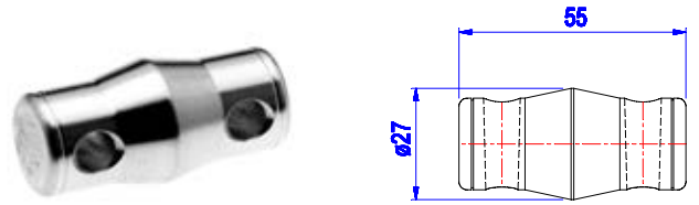
6011-002-001 ( 601111 ) MALE CONNECTION
