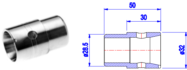
6011-001-001 ( 601110 ) FEMALE CONNECTION
